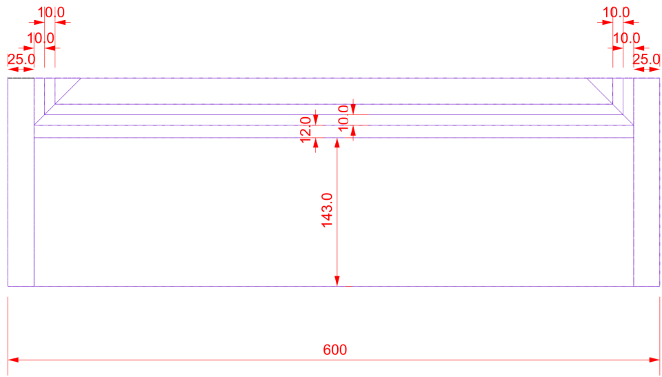
SKIRTING TO ARCHITRAVE TRANSITION WITH 12mm SHADOW GAP TO SUIT 15mm BOARD WITH PLASTER SKIM
