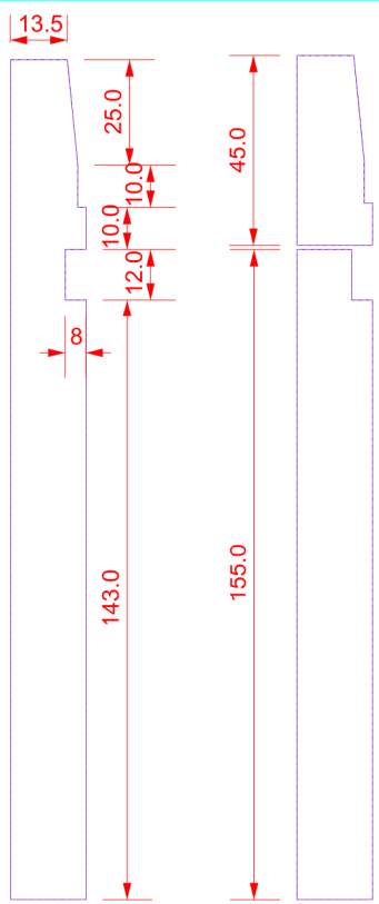
SECTION OF STANDARD SKIRTING & SPLIT SKIRTING
