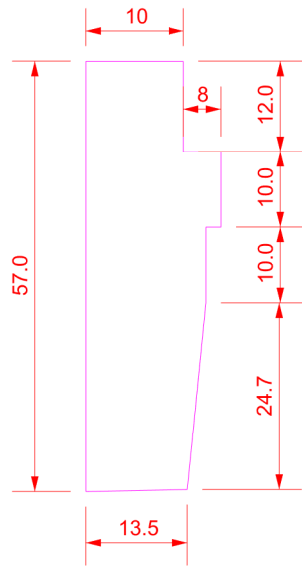
SECTION OF STANDARD SKIRTING & SPLIT SKIRTING
