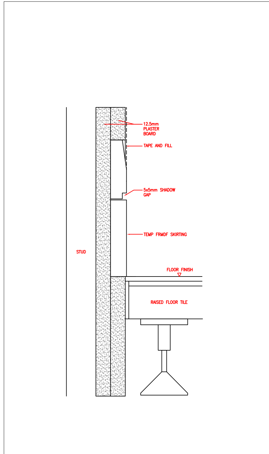
SHOWING TEMP SKIRTING 1:2 @ A1
