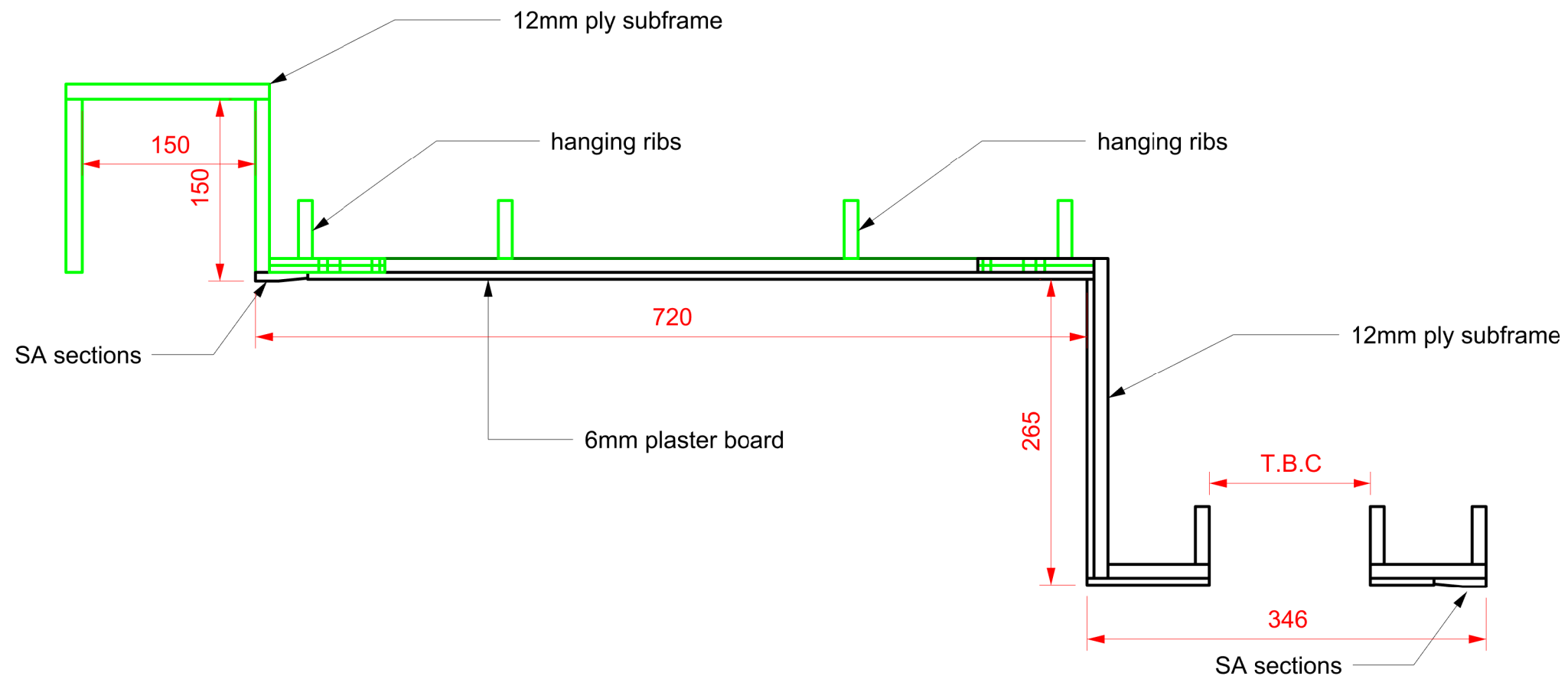
Section Through
