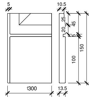
SA-14 (150/5x5)R (300mm length)
