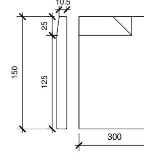
SA-14 (150/5x5)L (300mm length)
