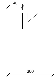
SA-15 (150/40x40)R (300mm length)
