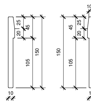
SKIRTING SA-15-40mm SA-15 (150/40x40) (3000mm length)
