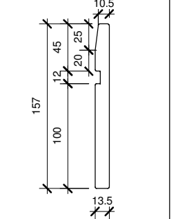
SKIRTING SA-14-12mm SA-14 (157/12x12) (3000mm length)
