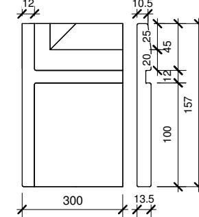
SA-14 (157/12x12)R (300mm length)
