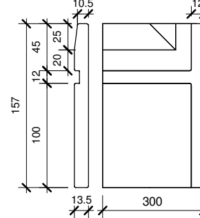
SA-14 (157/12x12)L (300mm length)
