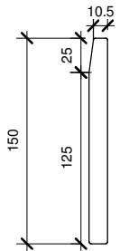
SKIRTING SA-14 SA-14 (150) (3000mm length)
