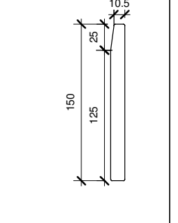
SKIRTING SA-14 SA-14 (150/5x5) (3000mm length)
