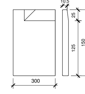
SA-14 (150/5x5)R (300mm length)
