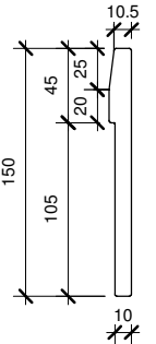
SKIRTING SA-15-40mm SA-15 (150/40x40) (3000mm length)
