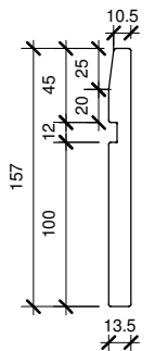
SKIRTING SA-14-12mm SA-14 (157/12x12) (3000mm length)
