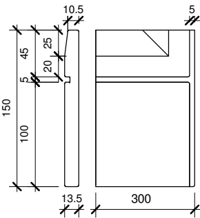
SA-14 (150/5x5)L (300mm length)
