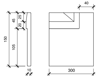
SA-15 (150/40x40)L (300mm length)
