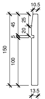
SKIRTING SA-14-5mm SA-14 (150/5x5) (3000mm length)
