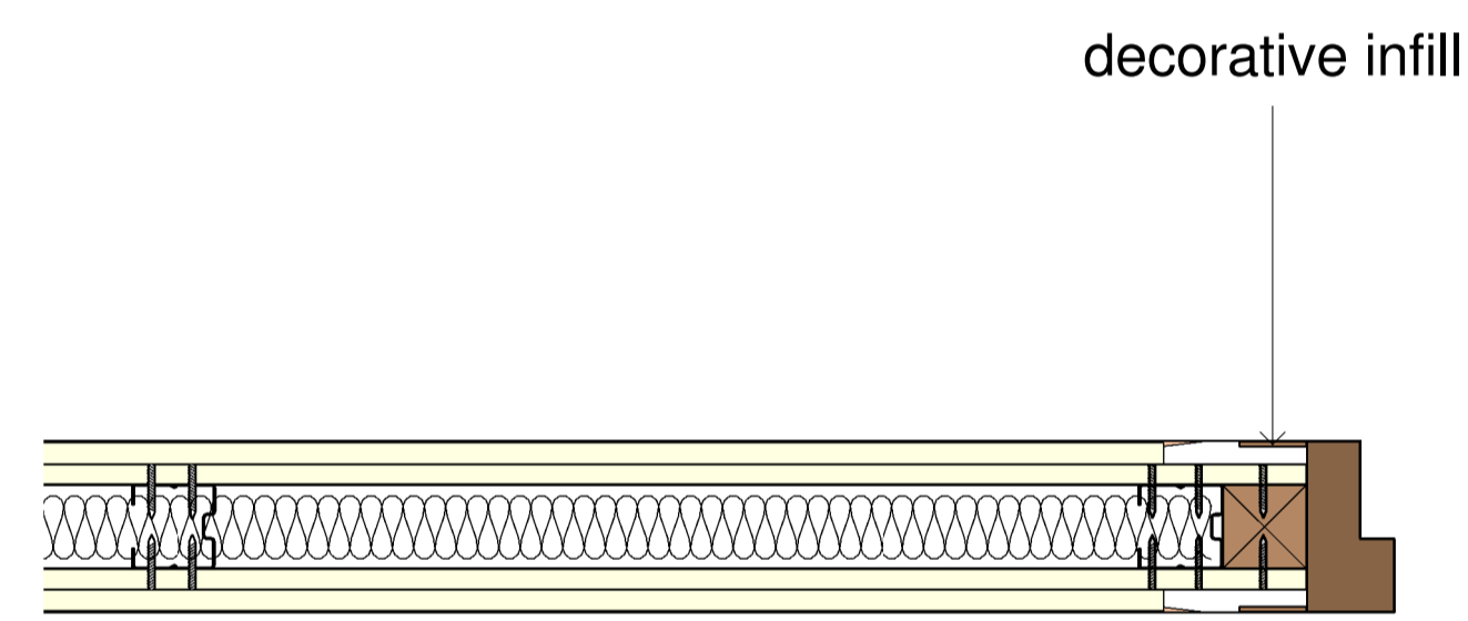
3 Architrave level - SA-16-40 1:5
