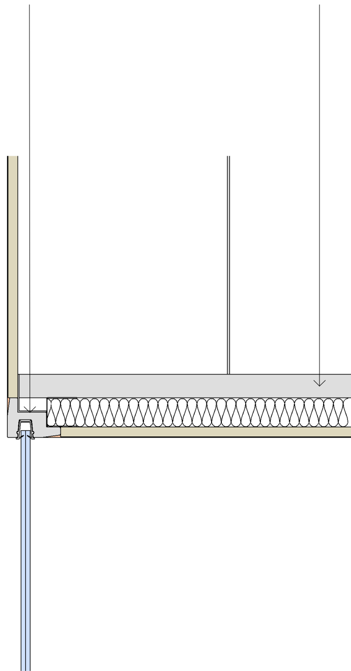
Profile for SA-17 ceiling system
