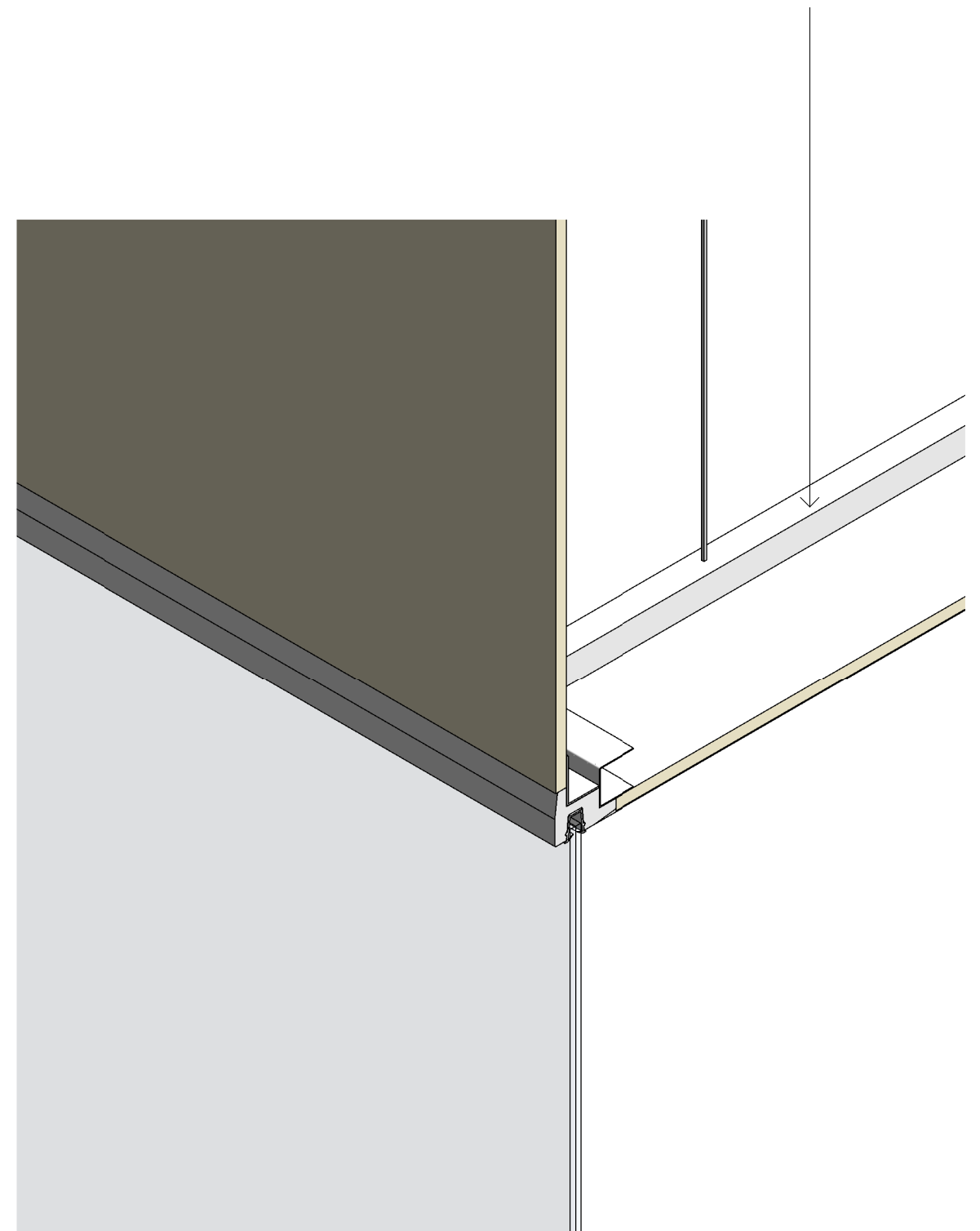
2 View, SA-17 ceiling system
