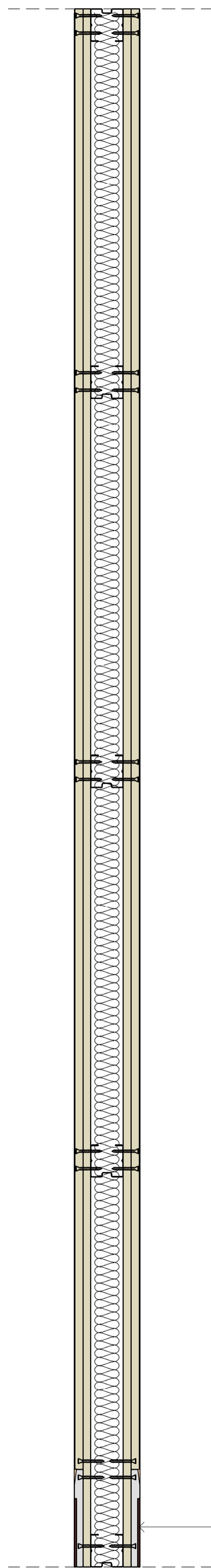
1 Section SA-15-150-40X40 1:5
