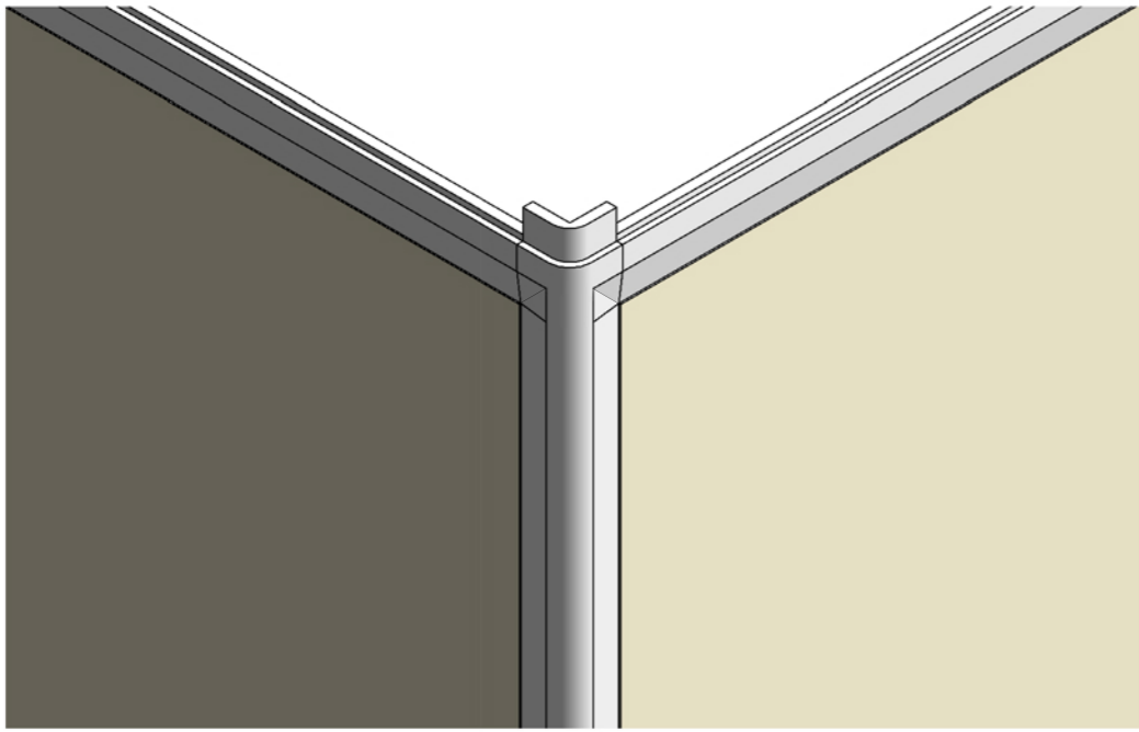
1 SA-11-45-45 r18 ext-40mm and SA-13-50-5
