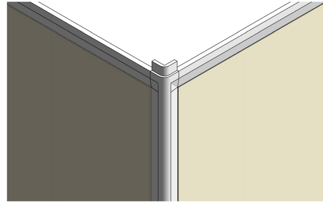
3 SA-11-45-45 r18 ext-no flash gap and SA-12-45
