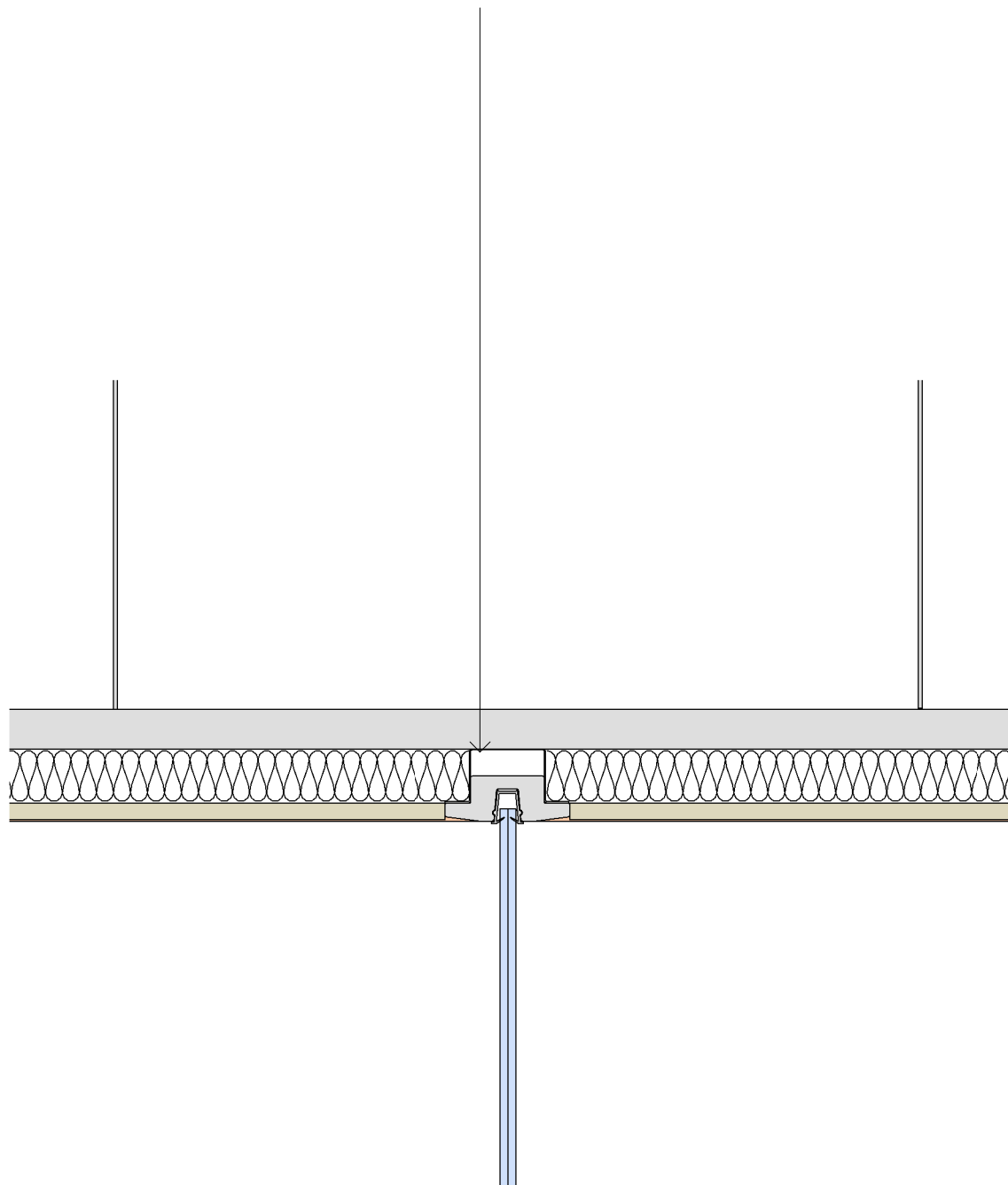
Profile for SA-1 ceiling system
