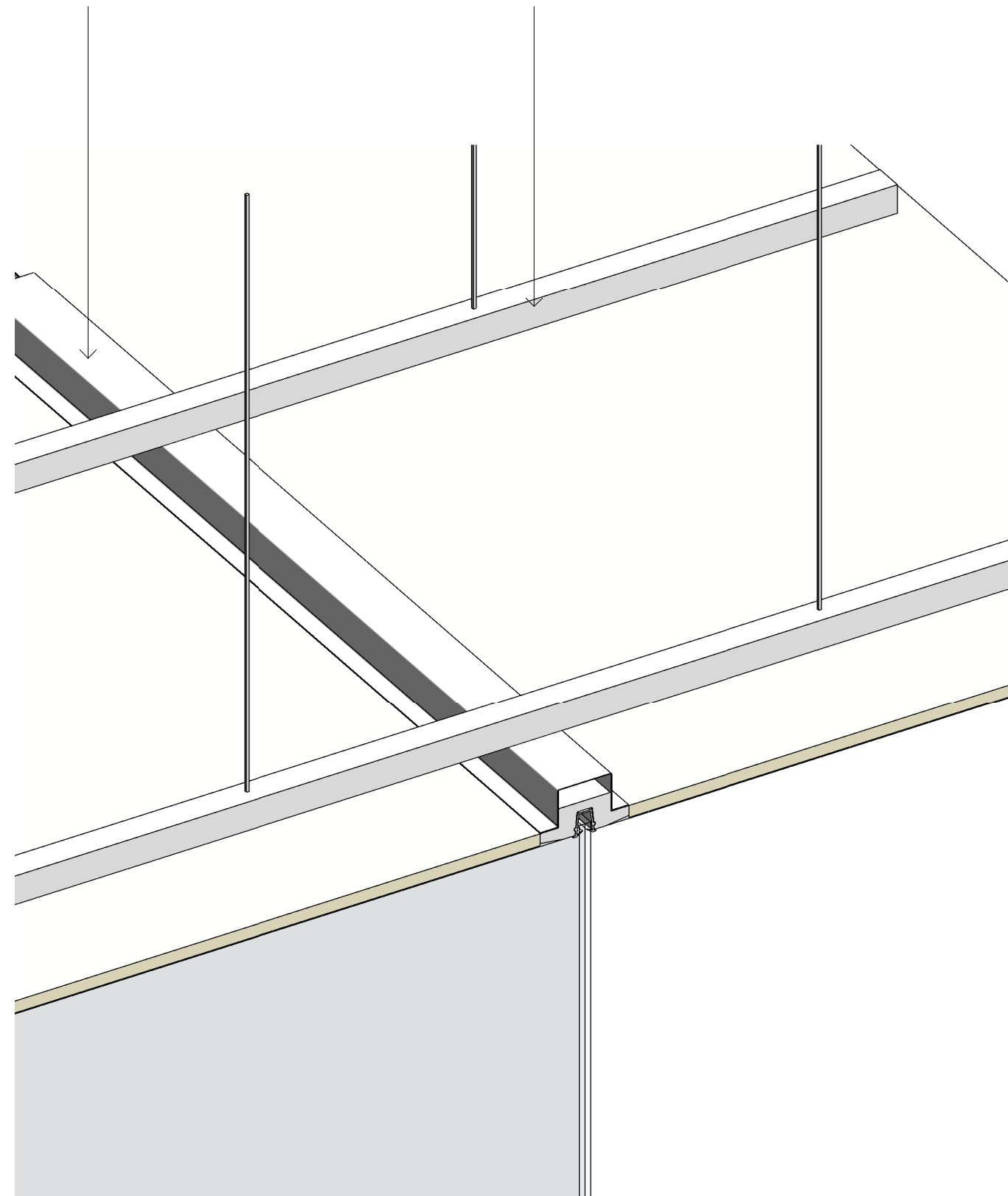
Profile for SA-1 ceiling system
